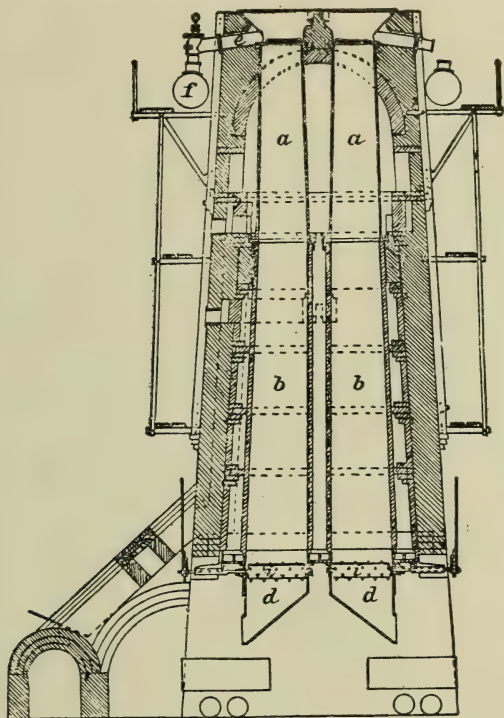
FIG. 85.—Henderson Retort for Distilling Shales.
